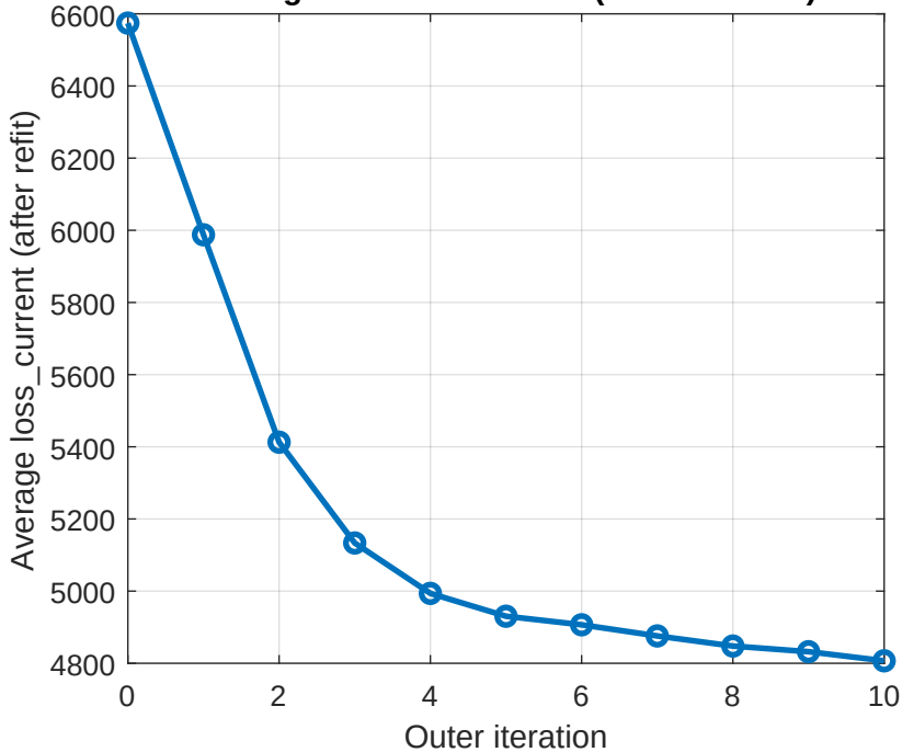
Average Loss vs Iteration (All Locations)
